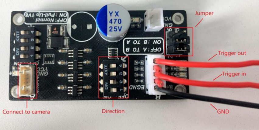
Camera Trigger Connection 1
