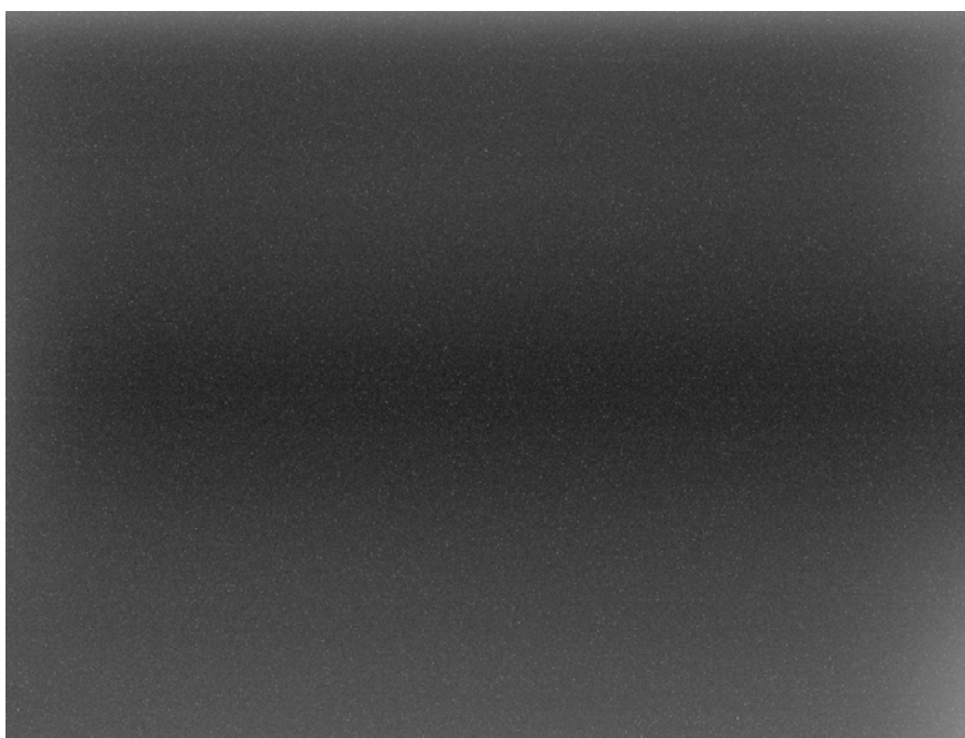
Amp Glow for an exposure of 600 secondi @ -10°C (STF stretch with PixInsight)
