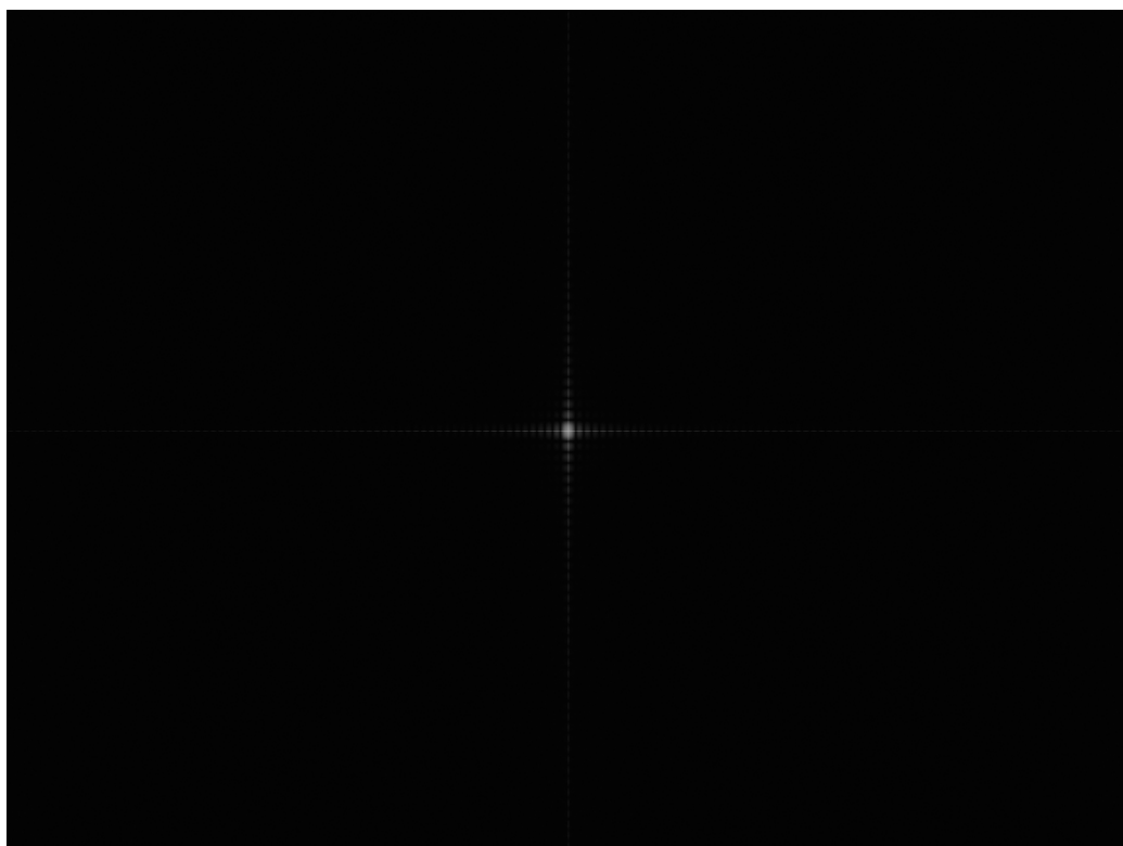
DFT of bias frame of a QHY163M
