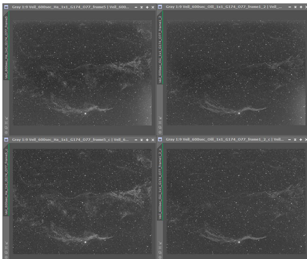
Removal of amp glow through calibration (with bias, dark and flat frames). Top row: uncalibrated light frames (left H-alpha, right O-III). Bottom row: the calibrated version of the same frames.
